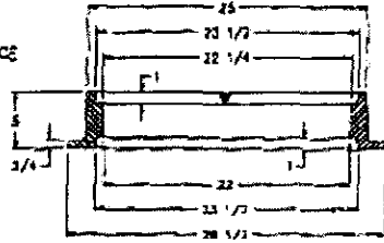
REVERSIBLE FRAME SECTION
