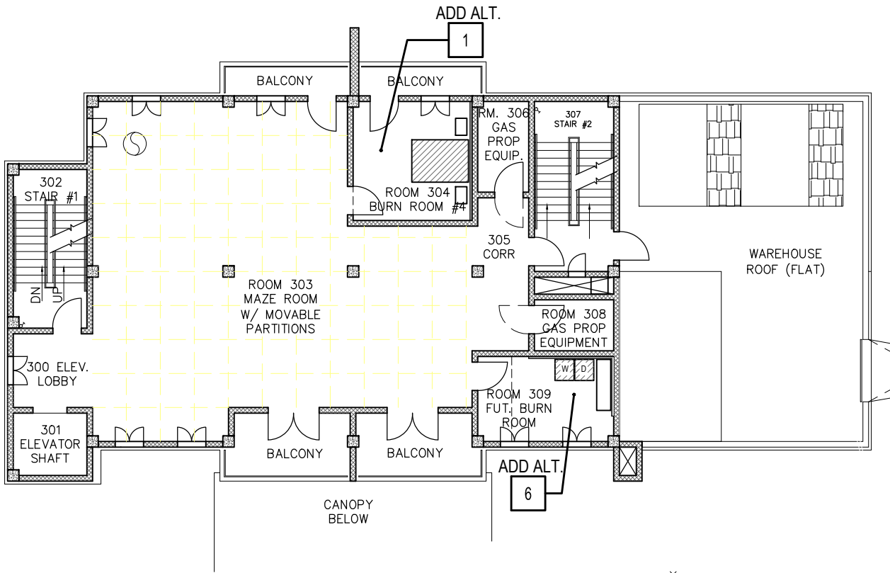
DRILL TOWER - THIRD FLOOR PLAN
