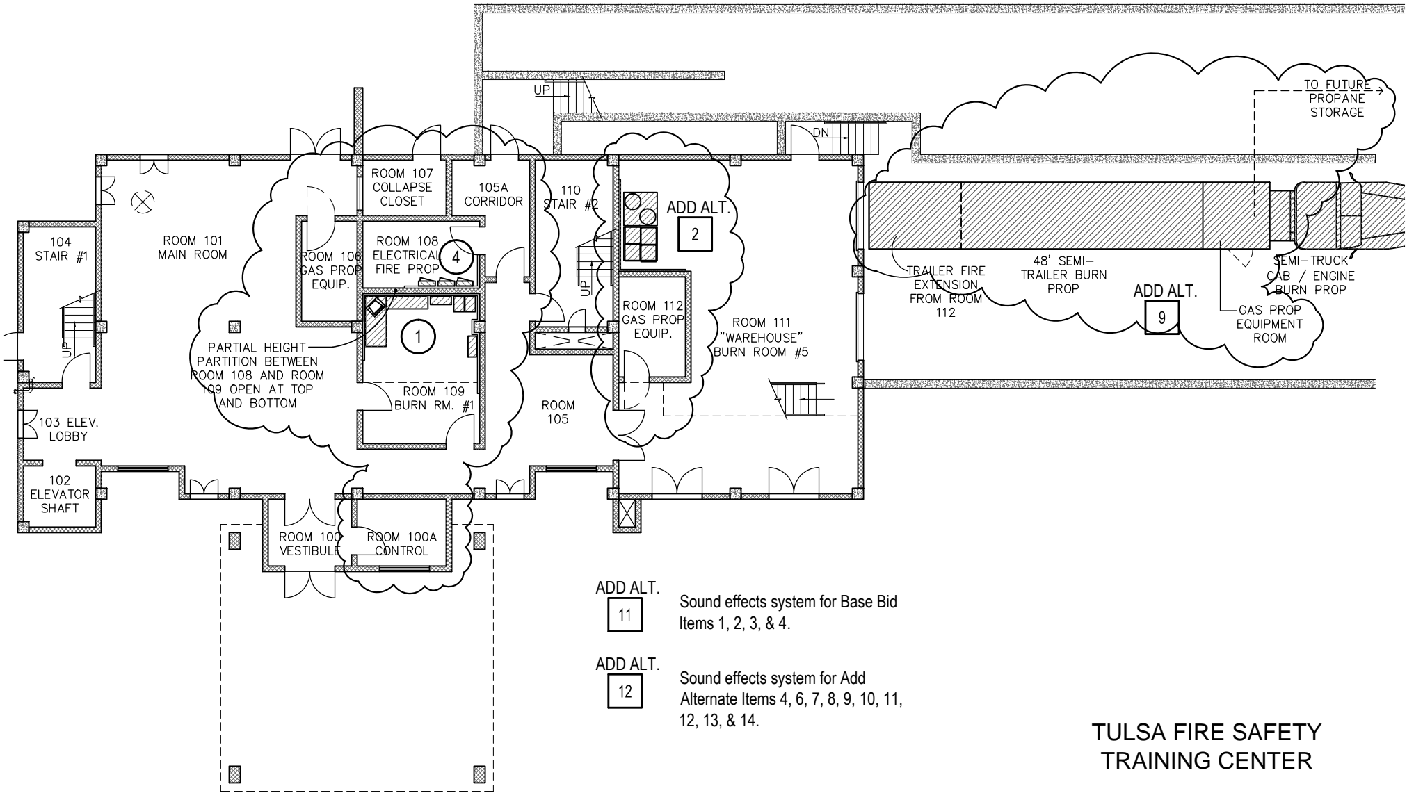
DRILL TOWER - FIRST FLOOR PLAN
