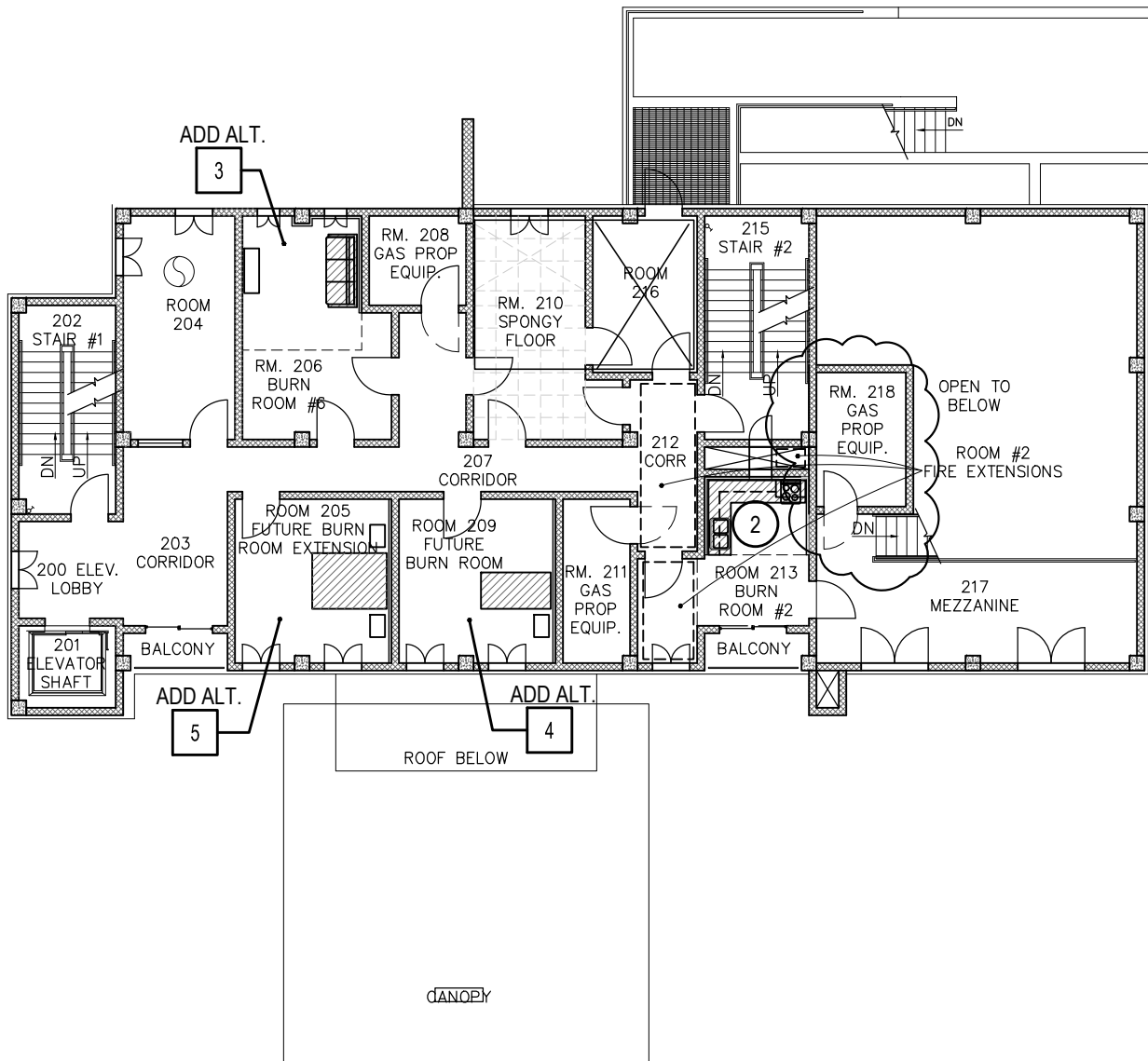
DRILL TOWER - SECOND FLOOR PLAN
