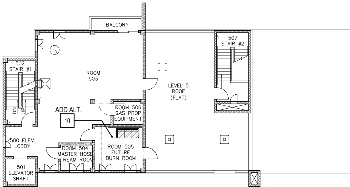
DRILL TOWER - FIFTH FLOOR PLAN
