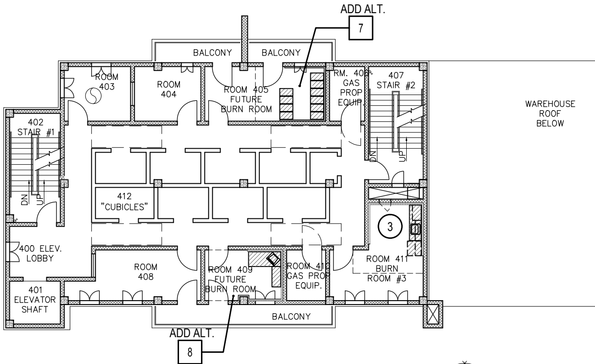
DRILL TOWER - FOURTH FLOOR PLAN
